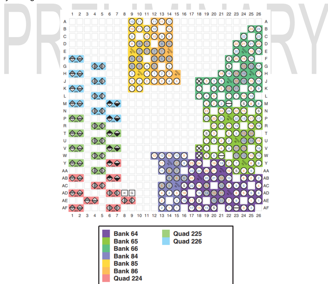
Figure 2 – FFVB676 Package Diagram
