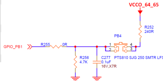
Figure 28 – User Push Buttons
