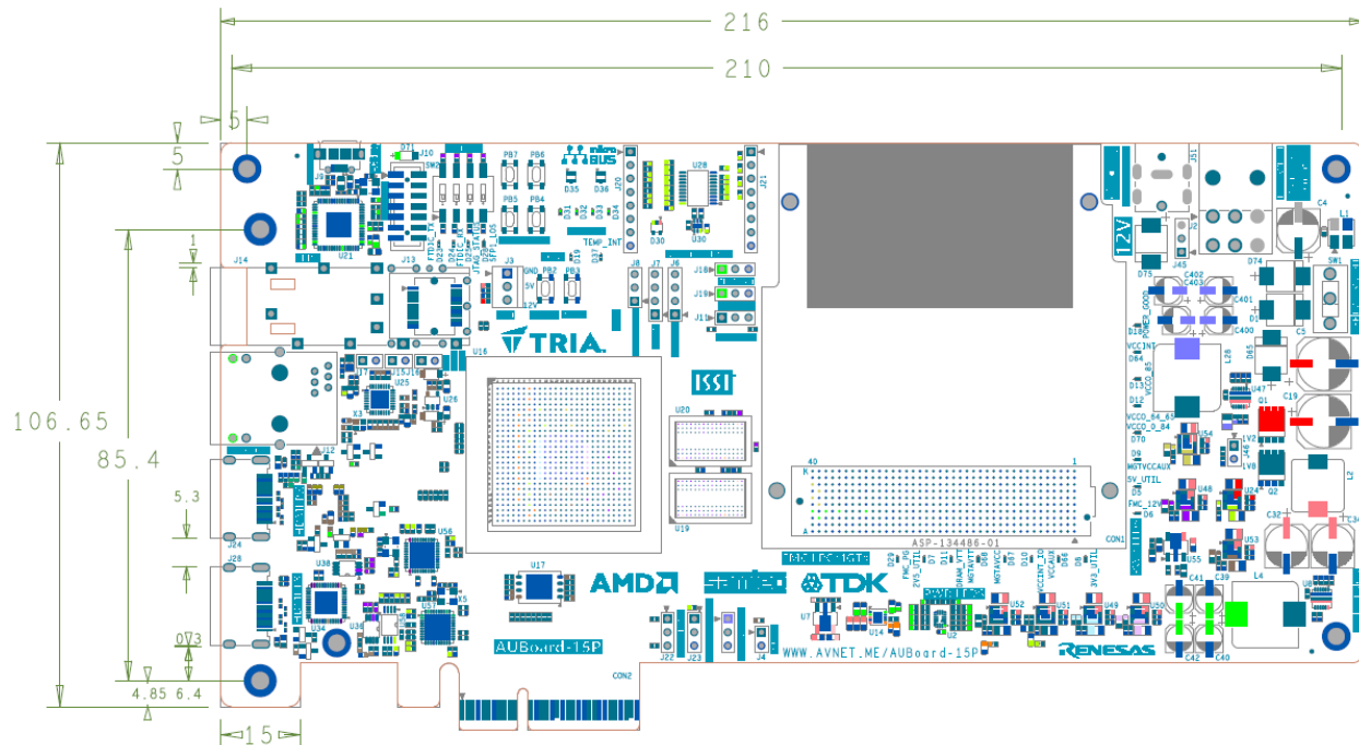
Figure 36 – Mechanical Dimensions
