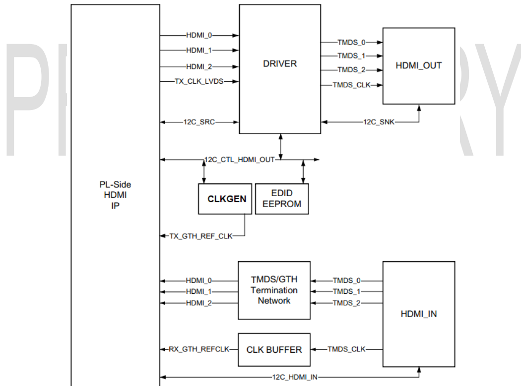
Figure 20 – HDMI Interface Block Diagram
