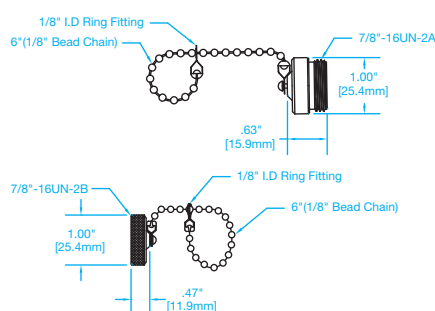
1300700018 (External Threads) and 1300700019 (Internal Threads)
